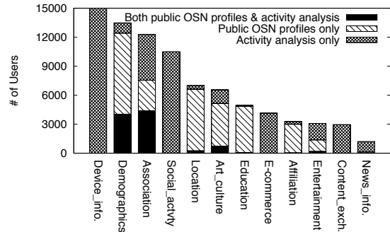
Figure 13: Personal info gathered from public OSN profiles, activity analysis on network trace, and both
