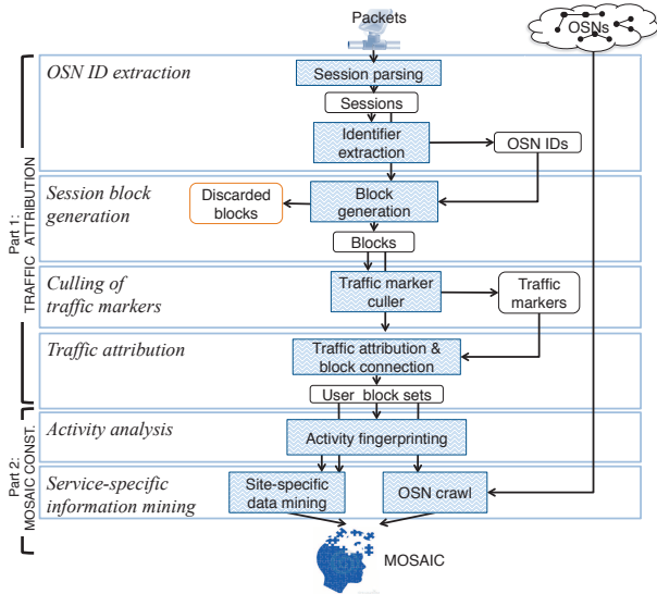
Figure 3: User mosaic construction via Tessellation
